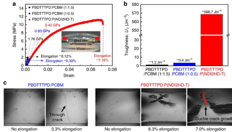
Figure 3. Tensile characterization of PBDTTTPD:PCBM and PBDTTTPD:P(NDI2HD-T) blended films: (a) stress–strain profiles; (b) comparison of the toughness for PBDTTTPD:PCBM and PBDTTTPD:P(NDI2HD-T) blends; (c) optical micrographs of PBDTTTPD:PCBM (1:0.5 w/w) and PBDTTTPD:P(NDI2HD-T) (1.3:1 w/w) blend films [2]
