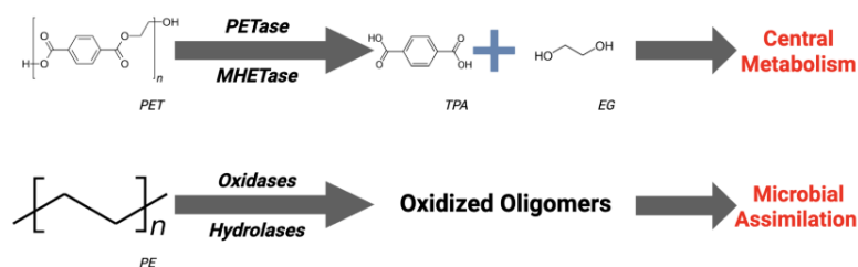
Figure 1. Microbial degradation of PET and PE
