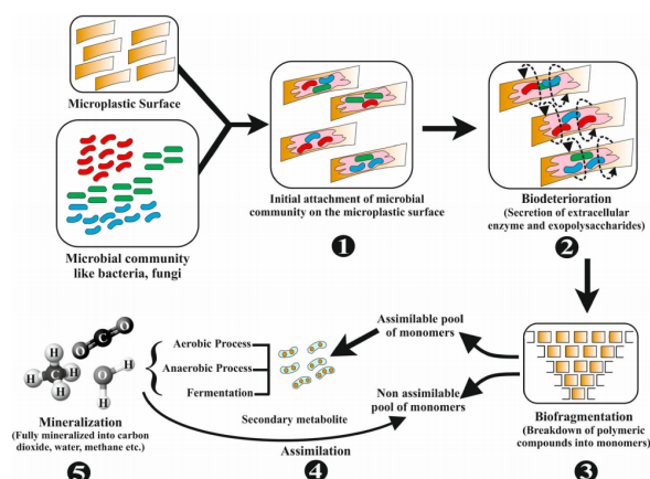
Figure 3. Schematic overview of microplastic biodegradation, showing microbial attachment, biodeterioration, biofragmentation, assimilation of monomers through aerobic or anaerobic processes, and final mineralization [28]
