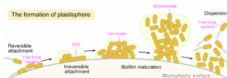
Figure 2. Stages of plastisphere formation on microplastic surfaces, including reversible and irreversible attachment, EPS secretion, biofilm maturation, and eventual dispersion of cells [27]
