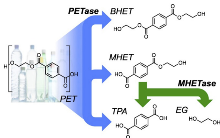
Figure 4. Enzymatic hydrolysis of PET. PETase converts PET into BHET and MHET, while MHETase further hydrolyzes MHET into terephthalic acid (TPA) and ethylene glycol (EG) [22]
