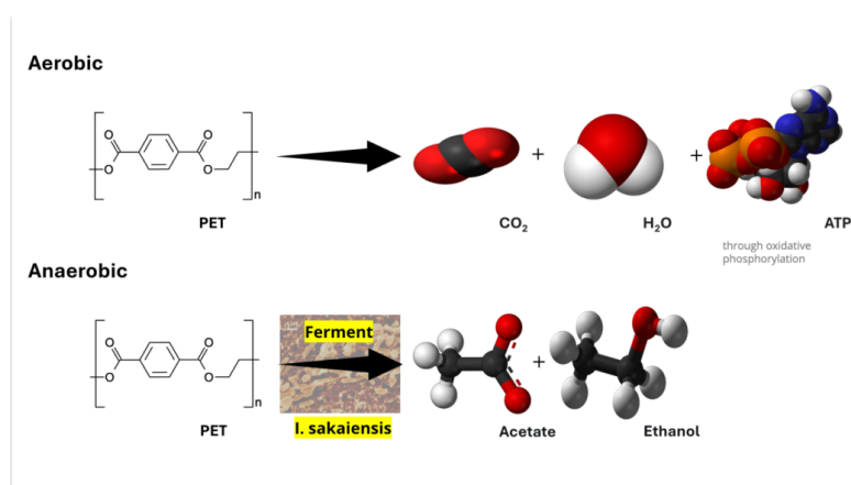
Figure 5. Aerobic versus anaerobic PET metabolism. Under aerobic conditions, PET is oxidized to \text{CO}_2 and \text{H}_2\text{O} with ATP generation, while under anaerobic conditions it is fermented by I. sakaiensis into acetate and ethanol
