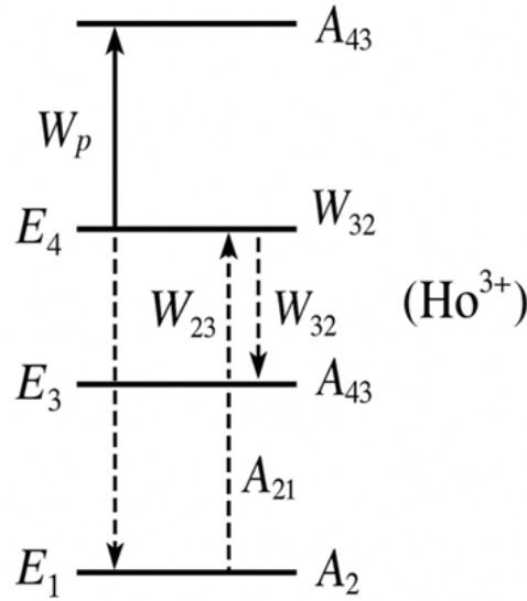
Figure 2. Simplified four-level model for \text{Ho}^{3+} laser transitions
