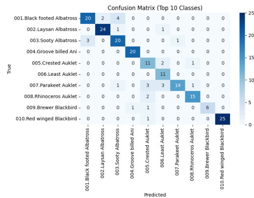
Figure 3. CLIP fine-tune
