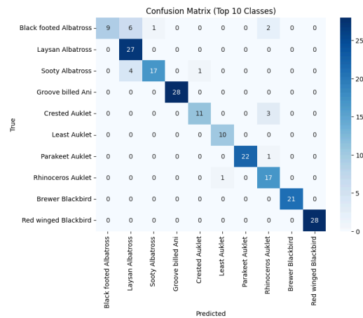
Figure 4. Swin fine-tune
