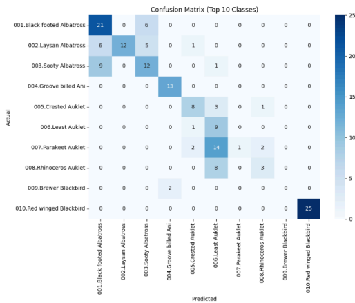
Figure 1. CLIP zero-shot
