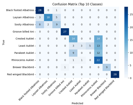
Figure 2. LiT zero-shot
