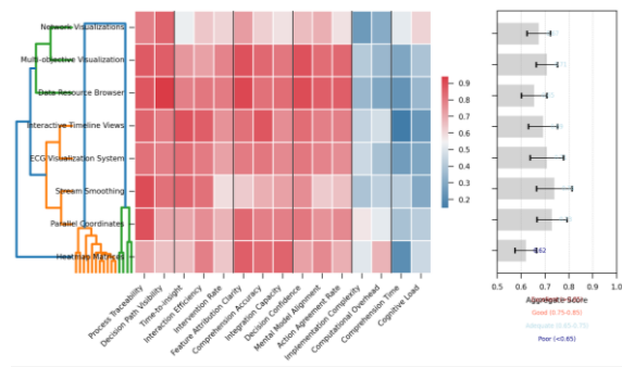
Figure 2: Heat Map Visualization of Transparency Performance Across Techniques
