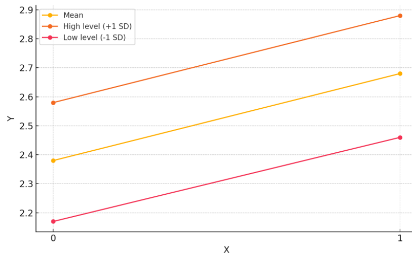
Figure 2. Simple slopes
