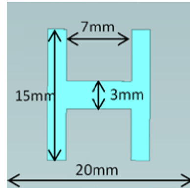
(b) Dimensions of FSS unit cell
