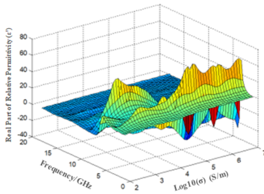
(a) Real part of permittivity
