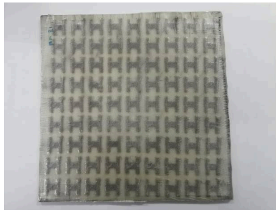
Figure 11. Photograph of laminated composite containing conductive fiber FSS material
