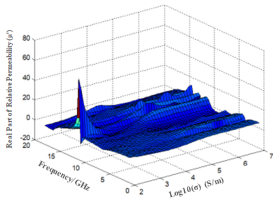
(c) Real part of permeability
