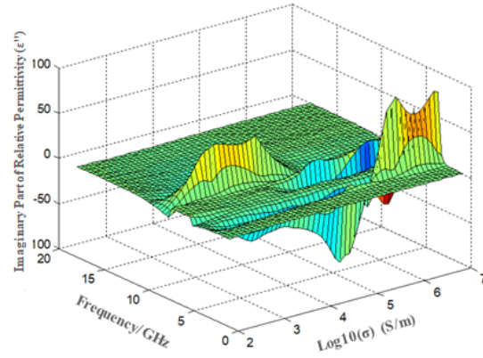
(b) Imaginary part of permittivity
